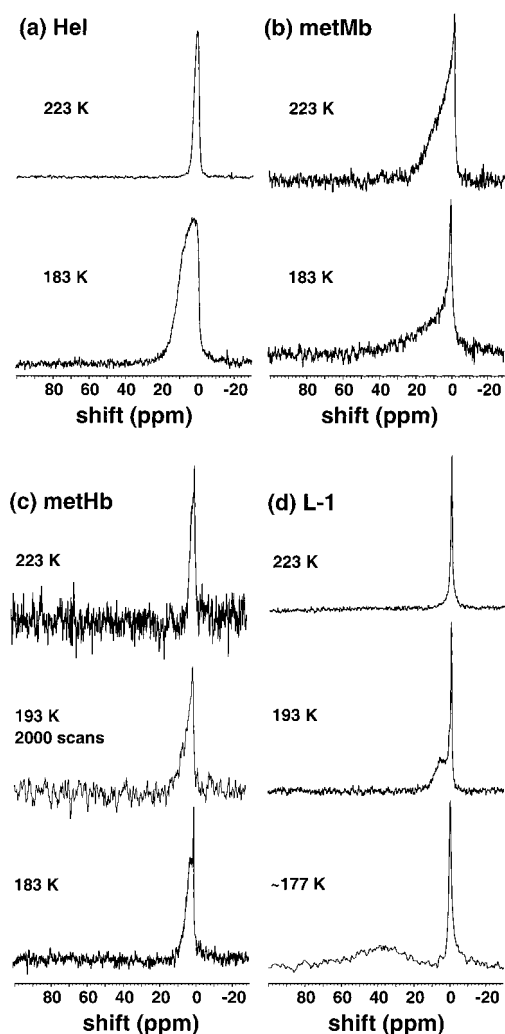
Figure 3. Hyperpolarized ^{129}\text{Xe} NMR study of Xe adsorption on 100–150 mg samples of lyophilized powders of (a) hen egg white lysozyme (Hel), (b) metmyoglobin (metMb), (c) methemoglobin (metHb), and (d) soybean lipoxygenase (L-1) at several temperatures, as indicated. The spectra have been normalized to the maximum intensity in each spectrum, and no correction has been applied to account for the loss of xenon spin magnetization by spin lattice relaxation or rf pulses. Except for the the 193 K spectrum of part (c), the ^{129}\text{Xe} NMR spectra were all recorded at 138.4 MHz using a single 45^\circ pulse (20- \mu\text{s} pulse width) in the presence of hyperpolarized xenon gas at a pressure equivalent to 2.0 atm at room temperature. The samples were thermally equilibrated for several minutes prior to acquisition. The 193 K spectrum of (c) is a conventional (field-polarized) ^{129}\text{Xe} NMR spectrum acquired at 110.7 MHz by signal averaging 2000 FIDs with a 1-s recycle delay.
