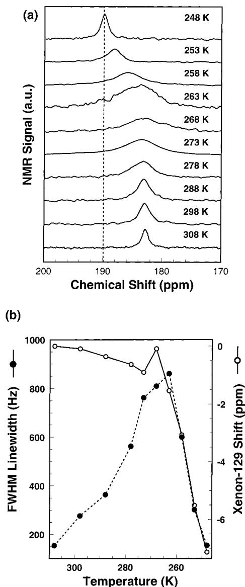
Figure 1. (a) Conventional ^{129}\text{Xe} NMR spectra, acquired as a function of temperature, of a solution containing 3.3 mM metMb in 0.50 mL of ethylene glycol, 0.50 mL of methanol, and 1.0 mL of \text{D}_2\text{O} . The 8.5-mL volume sample tube contained 2.2 atm of xenon. Fourier transformed spectra were acquired by signal averaging 6000 FIDs with a 500-ms recycle delay. (b) Summary of the temperature dependence of the ^{129}\text{Xe} NMR line widths (filled circles) and line shifts (open circles) in the metMb sample.
