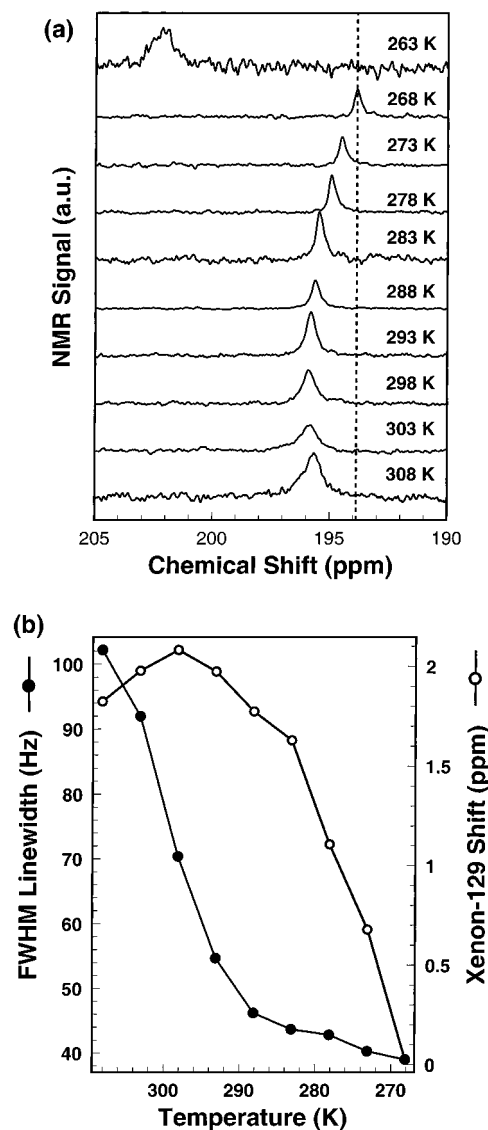
Figure 2. (a) Conventional ^{129}\text{Xe} NMR spectra of a 1 mL solution containing 50 mg of lipoxygenase, type L-1 from soybeans, dissolved in a 0.01 mM potassium cryoprotectant solvent (see text). The spectra were acquired as a function of temperature at a Xe pressure of approximately 1.7 atm. A total of 4000 FIDs were signal-averaged using a recycle delay of 500 ms. (b) Summary of the temperature dependence of the ^{129}\text{Xe} NMR line widths (filled circles) and line shifts (open circles) in the L-1 sample.
